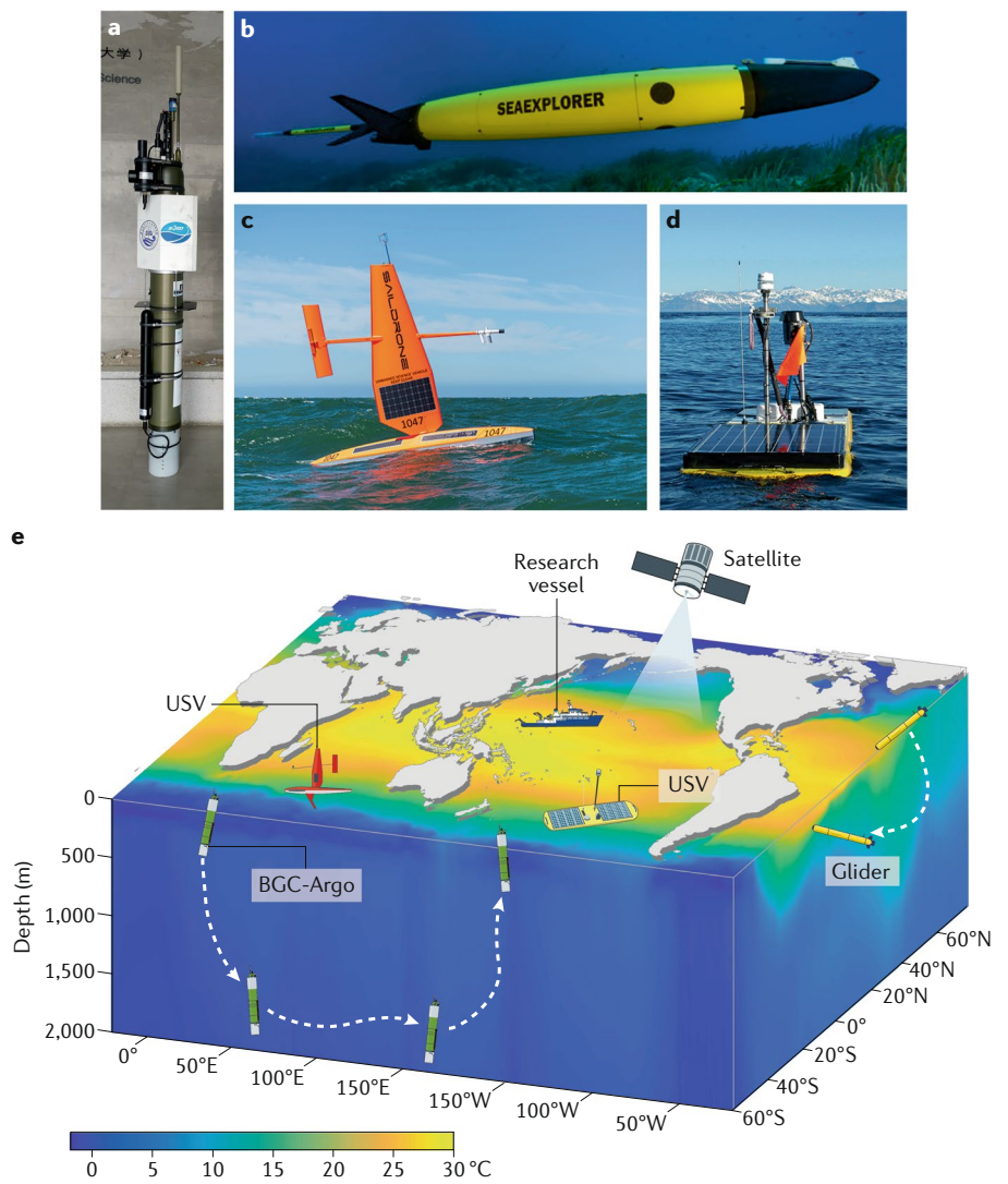
Fig. 3 | Four available ocean-observation platforms and example areas of operation. a | A typical Biogeochemical-Argo (BGC-Argo) float. b | A glider. c | A saildrone (a type of unmanned surface vehicle (USV)). d | A Wave Glider (a type of USV). e | A schematic diagram of ocean-observation-platform operations, along with research vessels and satellites. Traditional shipborne platforms provide fundamental reference data for many biogeochemical variables across all platforms, and satellite sensing provides the continuous spatiotemporal coverage of sea-surface variables. The Argo and BGC-Argo arrays measure ocean variables through the water column, with all floats reaching up to 2,000 m. Gliders are more suitable for observation at various depths in coastal and shallow oceans, whereas USVs provide air-sea flux data. Panel b reprinted with permission from ALSEAMAR. Panel c reprinted courtesy of Saildrone. Panel d reprinted with permission from NOAA PMEL/Evans (Hakai Institute).
