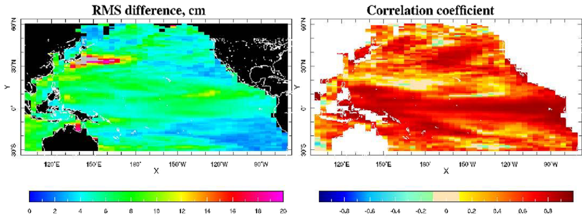
Fig. 10. Comparison for 4^\circ \times 1^\circ monthly means of the ROMS North Pacific simulation for 1996–2002 forced by daily fluxes from the NCEP–NCAR Reanalysis [52] with sea level heights from SSALTO/DUACS time-delayed merged altimetry maps [42].
